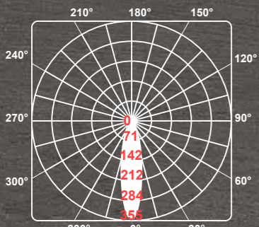
PHOTOMETRIC CURVE ALEA
